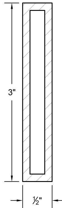
3" MIDRAIL
