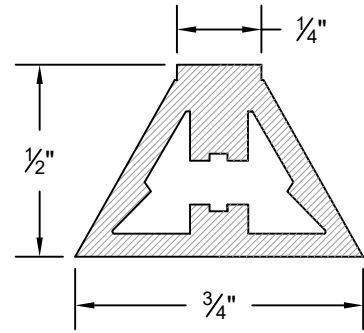
3/4" RAISED MUNTIN
