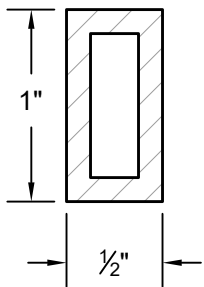
1" FLAT MUNTIN
