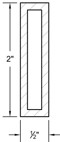
2" MIDRAIL
