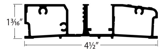
STANDARD SILL
