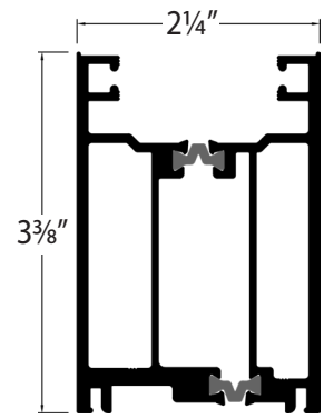
RECESSED STILE
