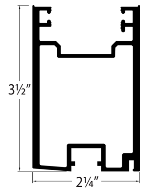
ACTIVE STILE
