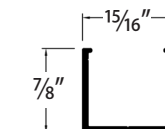
CHANNEL SILL
